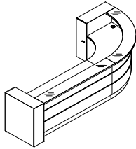
A: LAD10+LAP10+LA23L+NL41+LAV90L+LAL10+LAD10
