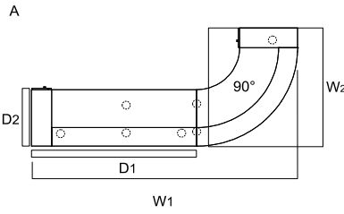
A: LAD10+LAP10+LA23L+NL41+LAV90L+LAL10+LAD10
