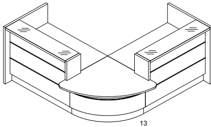
13 LAN1P+LA16L+NL41+LAN4L+LAV68L+NL41+LAN3P+LA23L+LAN2L 13 16
